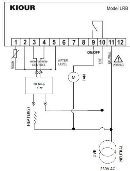
Heated cupboard
