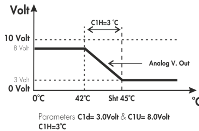
FIGURE 5B COMPRESSOR C1 HEATING MODE ANALOG OUTPUT OPERATION AND SETTINGS
