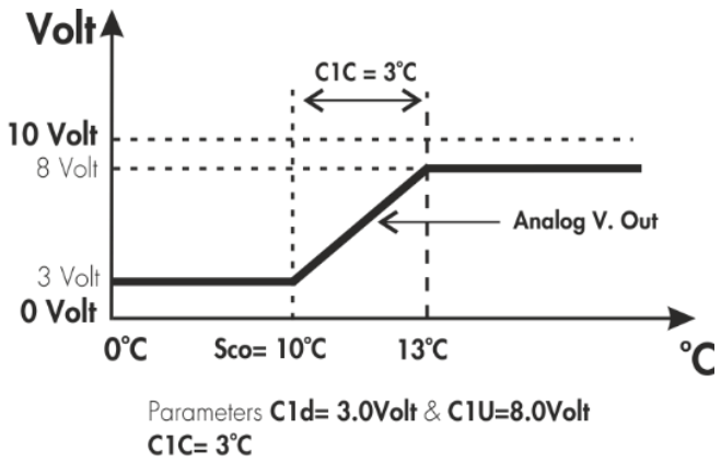
FIGURE 5B COMPRESSOR C1 HEATING MODE ANALOG OUTPUT OPERATION AND SETTINGS
