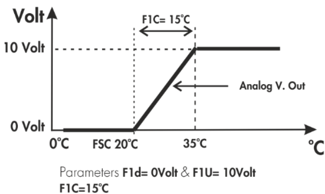
FIGURE 6B FAN 1 HEATING MODE SETTINGS
