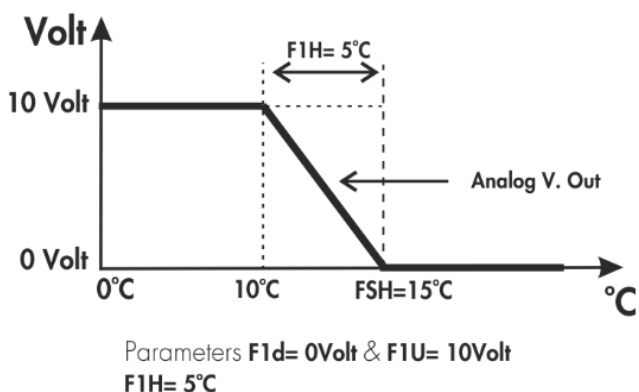
FIGURE 6B FAN 1 HEATING MODE SETTINGS
